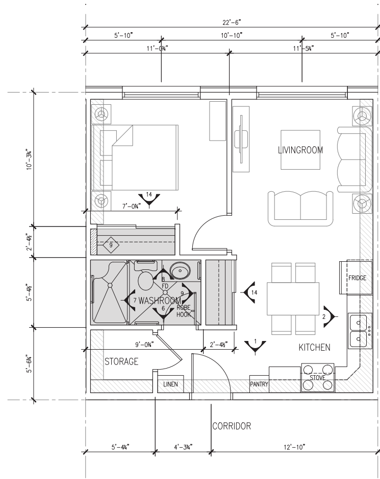
(35) A - UNITS Typical One Bedroom
