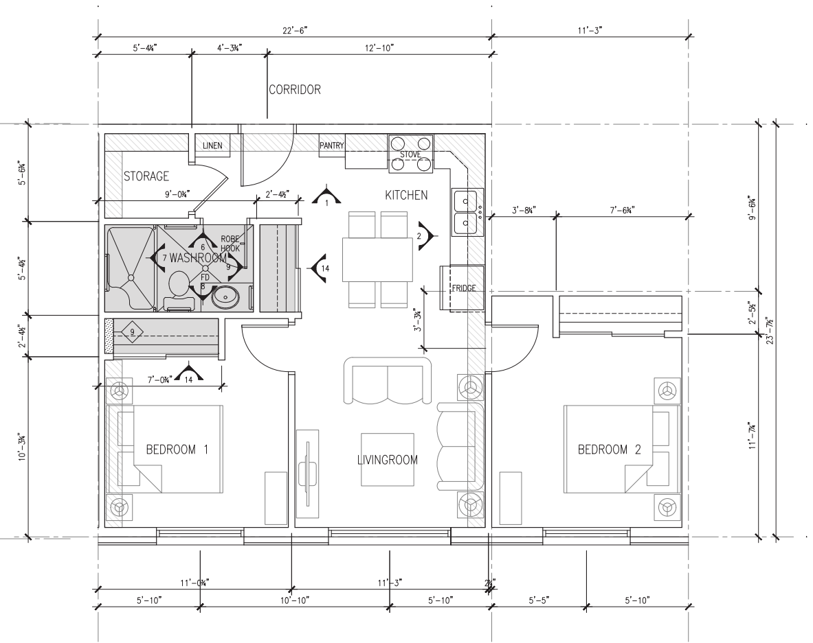
(3) C - UNITS Typical Two Bedrooms
