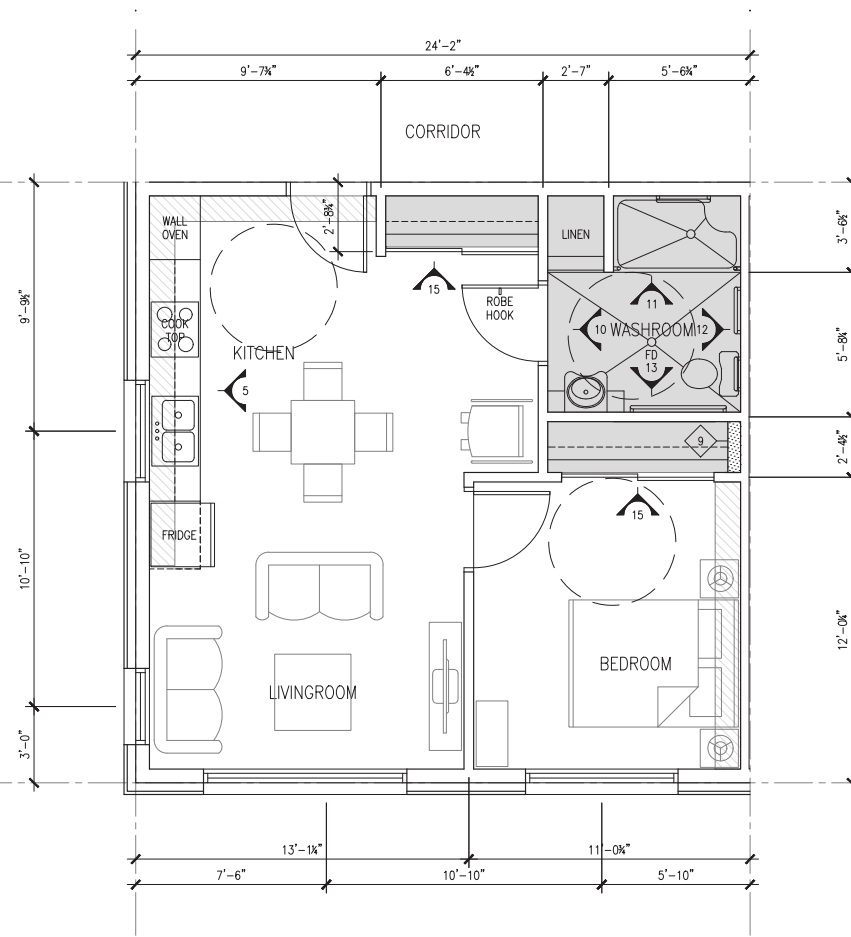
(10) B - UNITS Typical One Bedroom (Fully Accessible)
